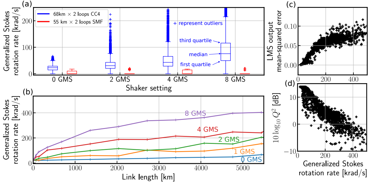
Fig. 2: (a) Distribution of the rotation rate of the generalized Stokes vector for a 68 \text{ km} \times 2 loop CC4 fiber and the rotation rate of the Stokes vector for a 55 \text{ km} \times 2 loop single-mode fiber, when both are perturbed by using a shaker operating at various shake strengths. (b) The rotation rate of the generalized Stokes vector for the CC4 fiber increases with the link distance. (c) The output instantaneous mean-squared error of the LMS equalizer is correlated with the instantaneous generalized Stokes rotation rate of the CC4 fiber. (d) Channel dynamics also impacts the received bit-error-rate and the derived Q^2 factors.
